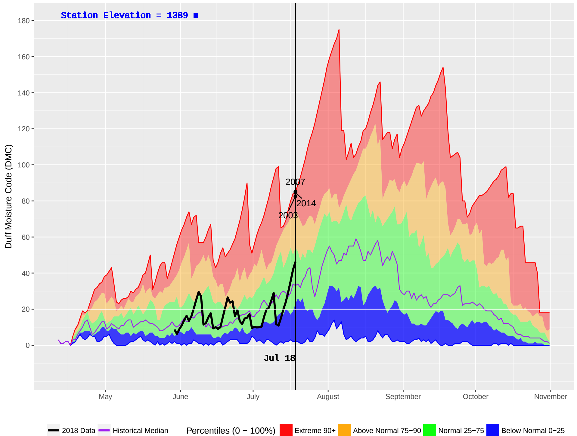
KETTLE 2 (388) : Historical (1987–2016) and Current (2018) Daily Duff Moisture Code (DMC)
