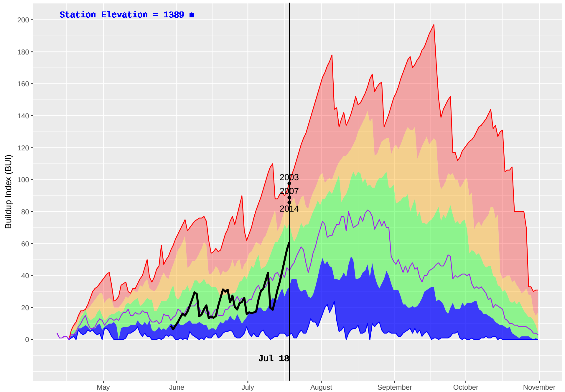
KETTLE 2 (388) : Historical (1987–2016) and Current (2018) Daily Buildup Index (BUI)
